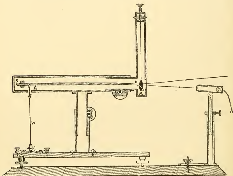
FIG. 49. The Magnetic Radiometer
