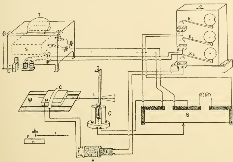
FIG. 29. The Self-recording Radiograph
