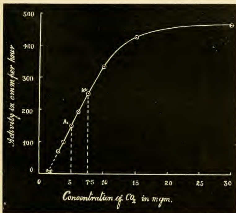
FIG. 58. Photosynthetic Curve under Variation of \text{CO}_2 -Concentration
