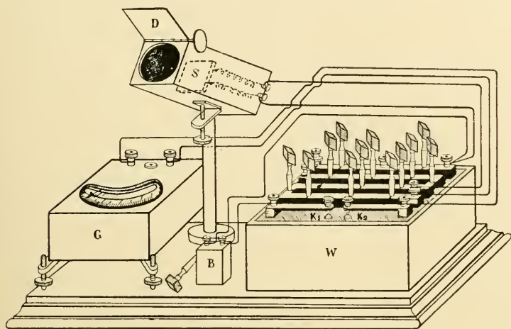
FIG. 32. The Portable Electric Photometer
