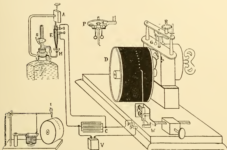
FIG. 3. The Automatic Recorder for Photosynthesis
