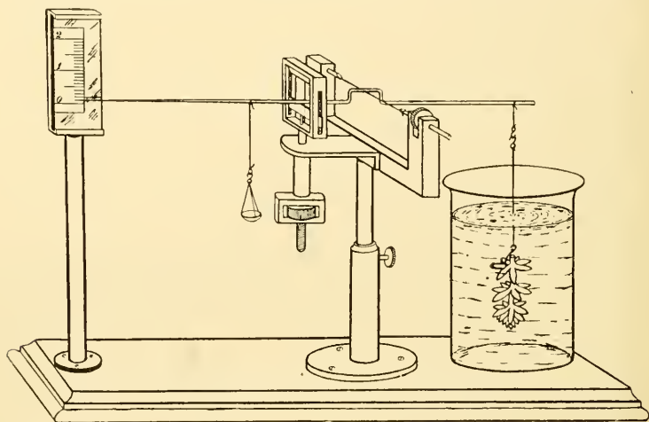
FIG. 52. The Torsion Balance for Measurement of Increase of Weight of the Living Plant during Photosynthesis
