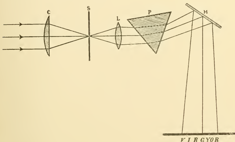
FIG. 48. Arrangement for obtaining a Pure Solar Spectrum
