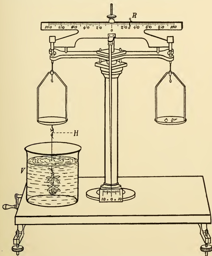
FIG. 53. Chemical Balance for determination of increase of weight of Hydrilla after exposure to Light.
