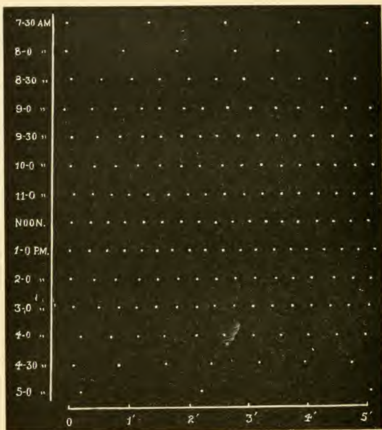
FIG. 44. Automatic Records of successive Bubblings for five minutes during different periods of the Day
