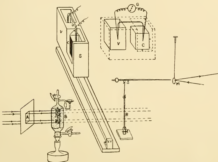
FIG. 55. Apparatus for Determination of Photosynthetic Efficiency
