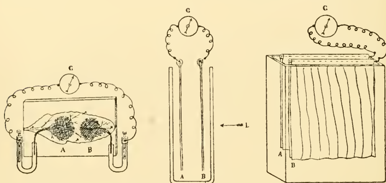
FIG. 18. Arrangement for obtaining Electric Response to Light The two figures to the right show the photo-electric cell.
