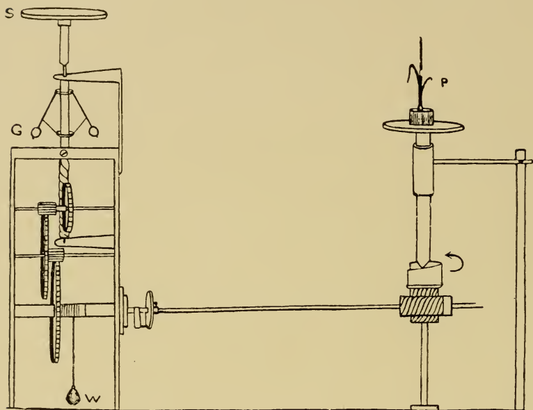
FIG. 9. Diagram of Method of Falling Weight.
