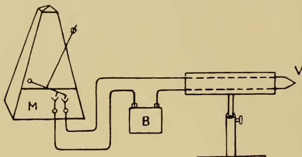
FIG. 100. Radio-Thermal Stimulator.
