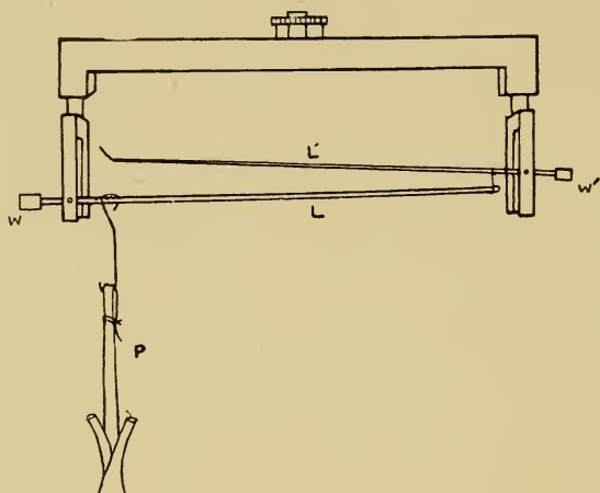
FIG. 1. Compound lever of High Magnification Crescograph.
