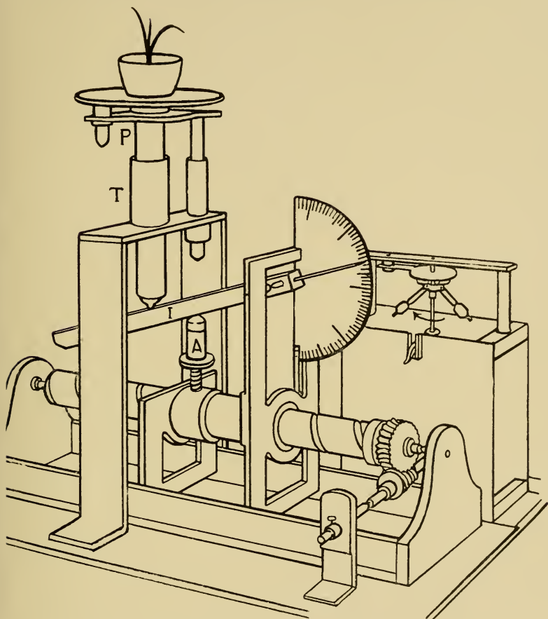
FIG. 12. The complete apparatus for Balance by Inclined Plane.
