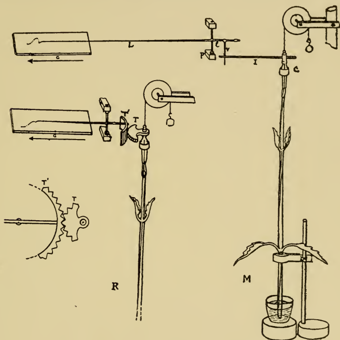
FIG. 218. Automatic Recorder of Torsion.
